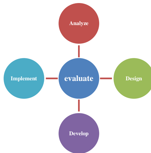
Gambar 1. Model ADDIE
