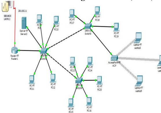
Gambar 7. Gedung B Lantai 2 (TSM)
