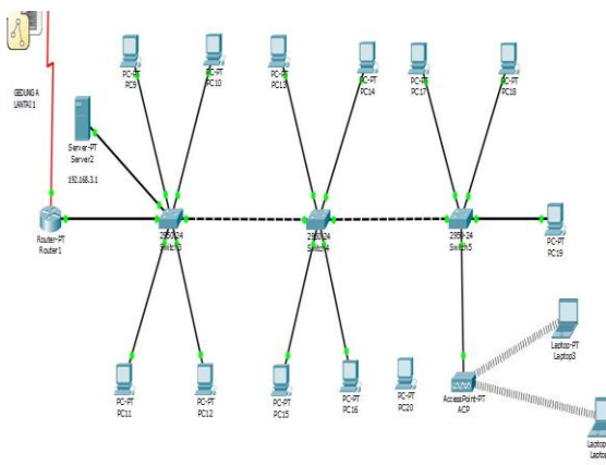
Gambar 5. Gedung A Lantai 2 (ACP)
